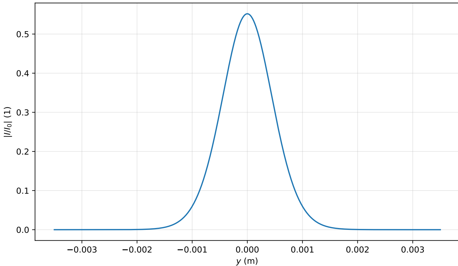
Intensity profile I(x=0, y, z=2.388)/I_0 , \text{Pin}=0.3\text{Pcr} , artificial time
